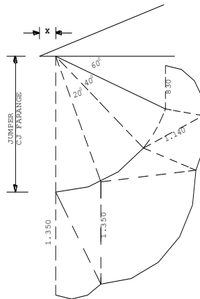
TENSION TOWER
