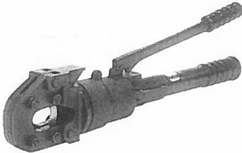
Fig. 1: Hand operated hydraulic wire cutter
