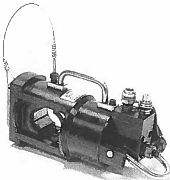
Fig. 3: Hand Operated Hydraulic Compression Tool of 400 - 1000mm 2
