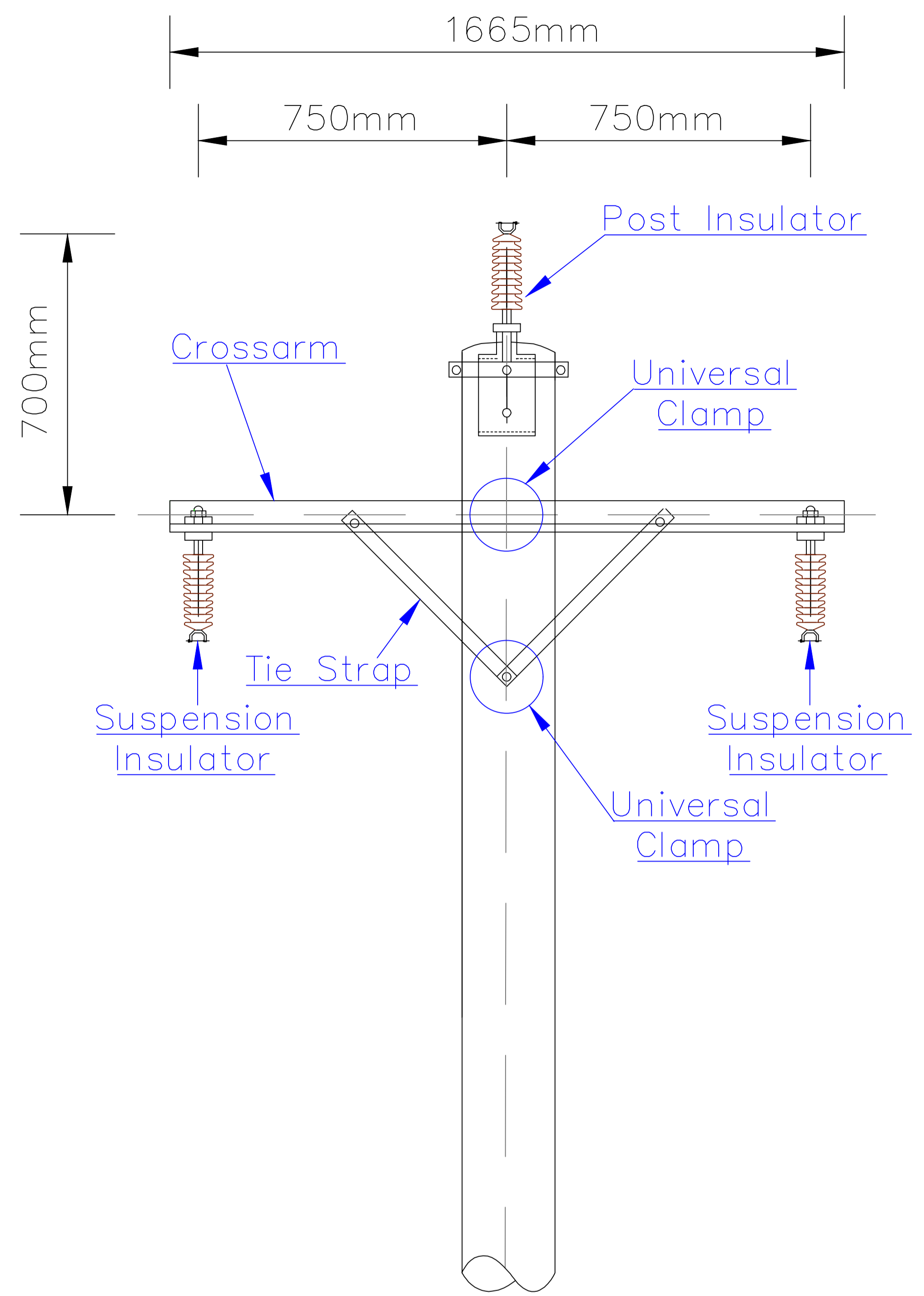
HORIZONTAL FORMATION FOR 11KV
