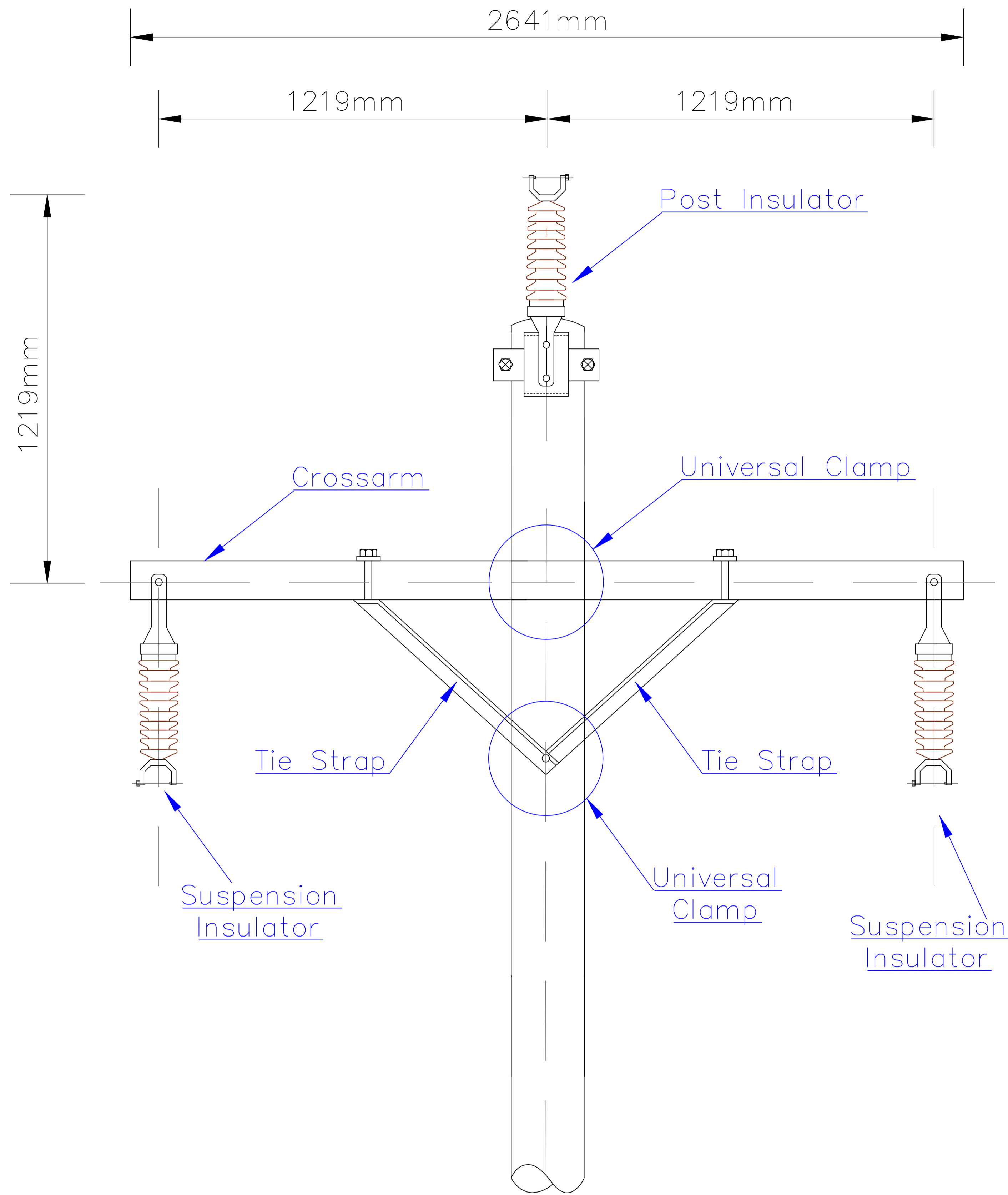
HORIZONTAL FORMATION FOR 33KV
