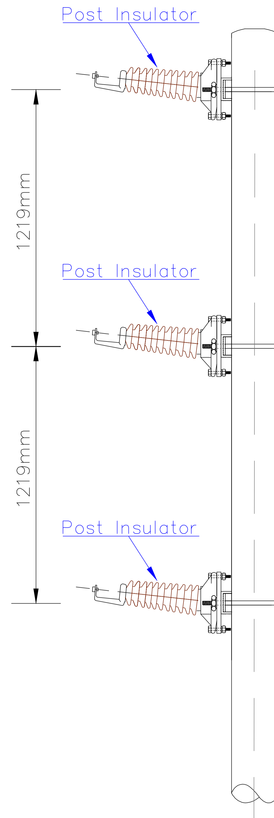
INTERMEDIATE VERTICAL FORMATION FOR 33KV
