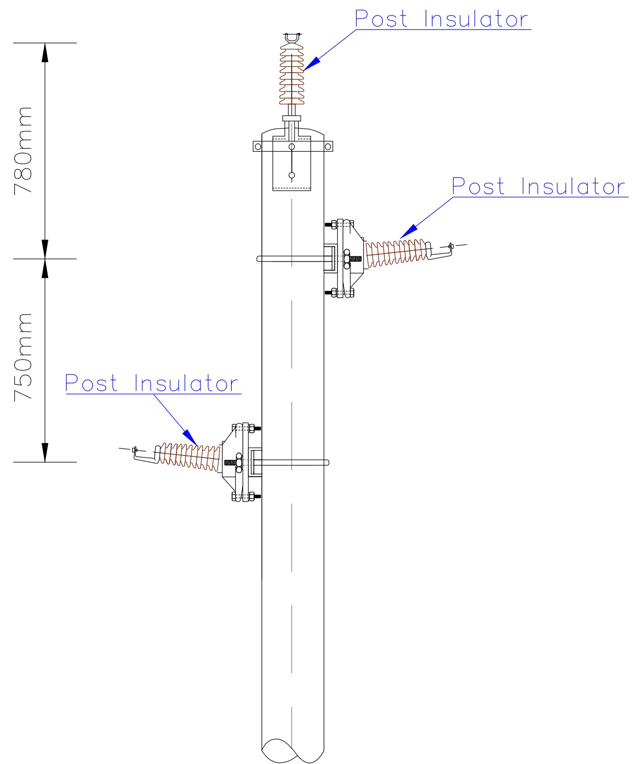
DELTA FORMATION FOR 11KV
