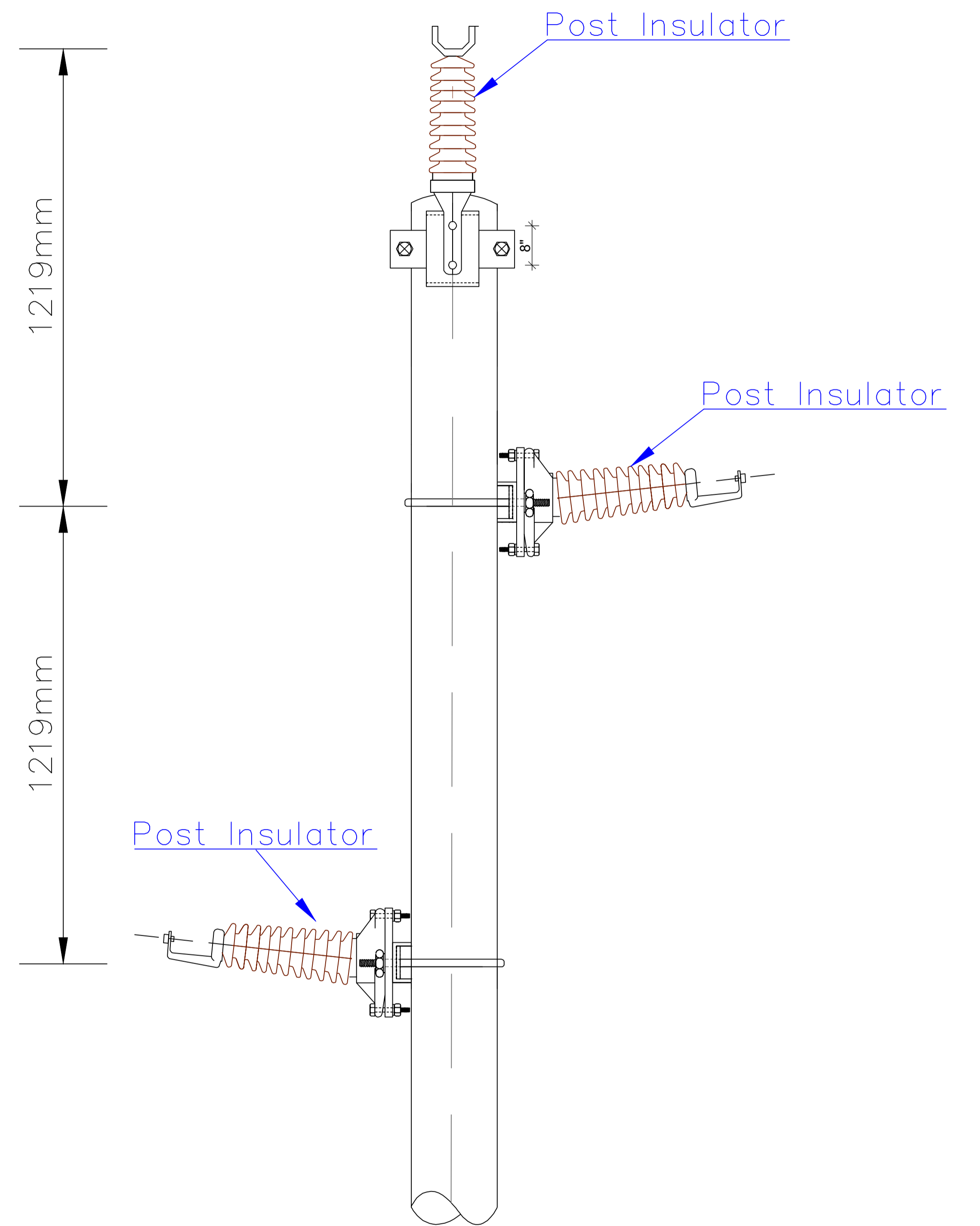
DELTA FORMATION FOR 33KV
